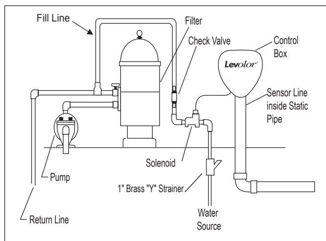
Figure 2. LX2 Installation
